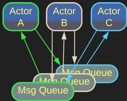
Actors
