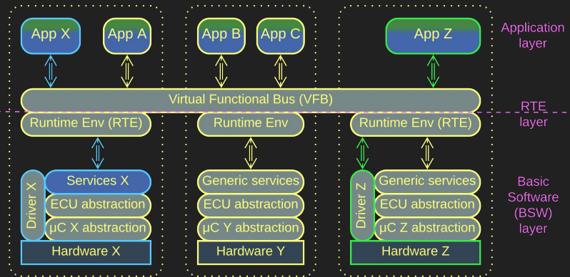
AUTOSAR Classic
