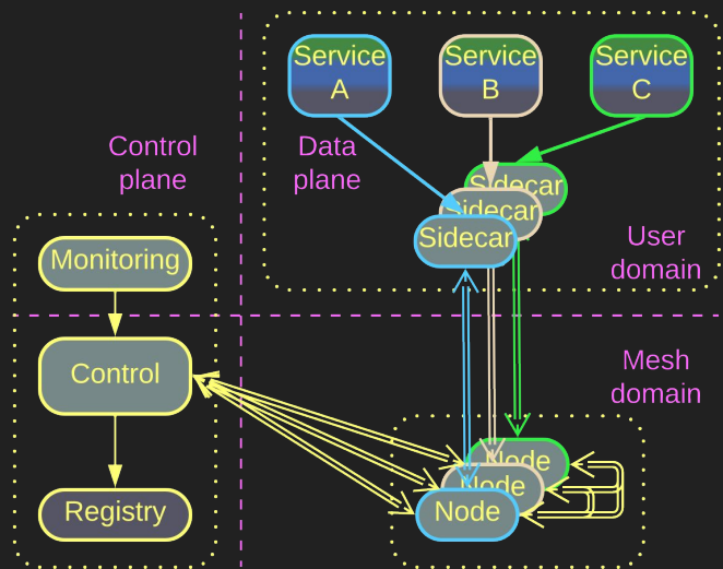
Service Mesh
