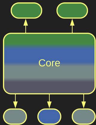
Plugins
