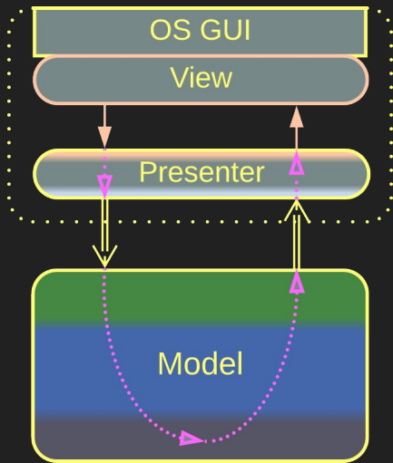
Model-View-Presenter
