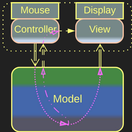
Model-View-Controller
