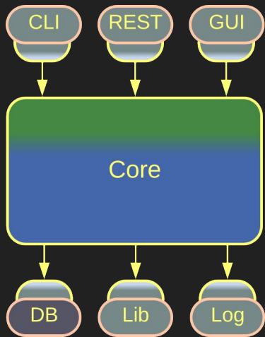
Hexagonal Architecture
