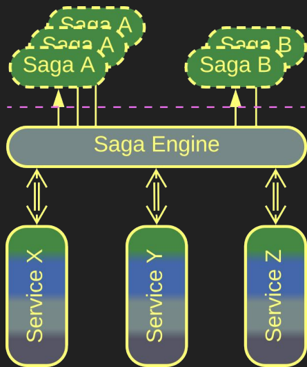
Saga Engine
