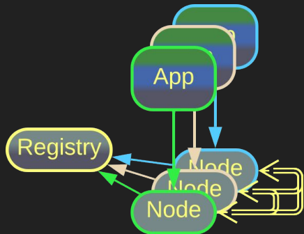
Peer-to-Peer Network
