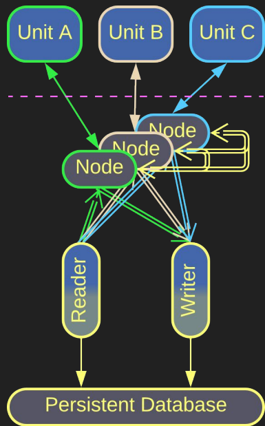
Space-Based Architecture
